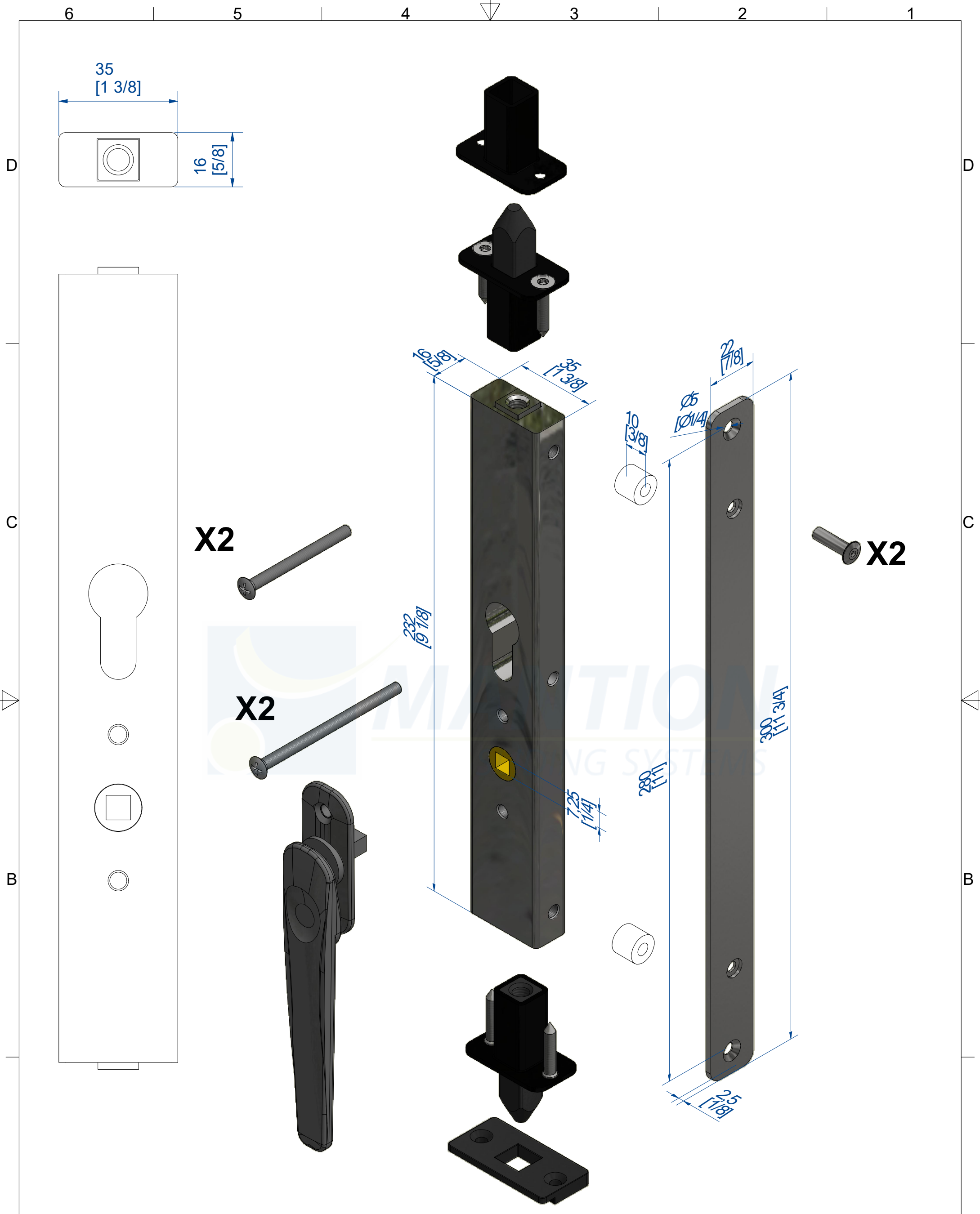
Set verrou 2 points et poignée Set 2 points bolt with handle
