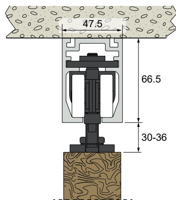
Wood mounting with plate 13044
