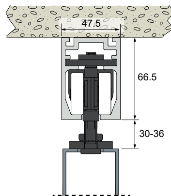
Metal mounting with plate 13044
