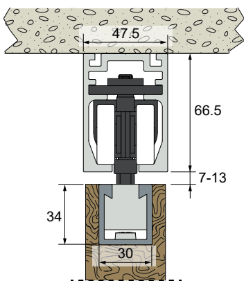
Wood mounting with plate 13040 + profile 28FC
