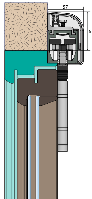
Wall mounting
