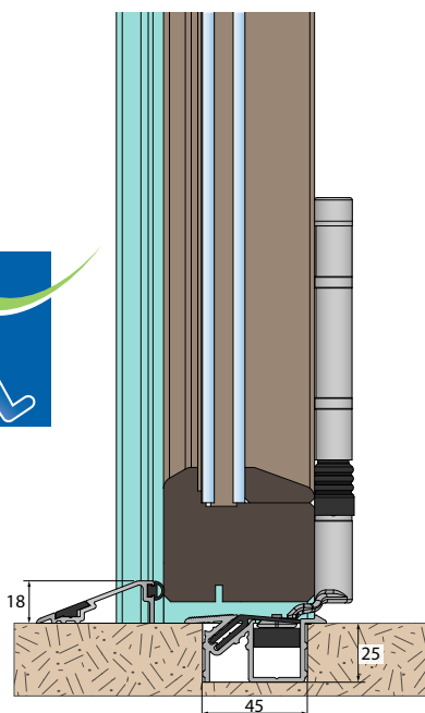
Flush-mounted threshold
