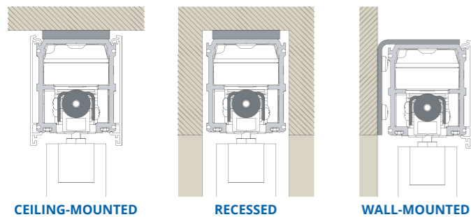
CEILING-MOUNTED
