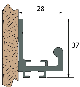
Rail SOFTCLOSE-GLOSS
