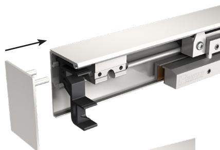
Rail fixation murale + bandeau
