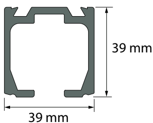
Rail 10300/... (2 - 3 - 6 m)
