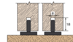
Montage 1103R + rainure
